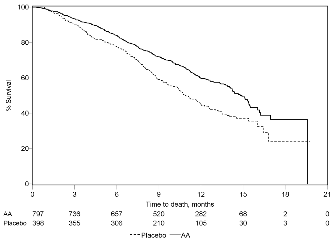
Figure6: Kaplan Meier survival curves of patients treated with either abiraterone or placebo in combination with prednisone or prednisolone plus LHRH analogues or prior orchiectomy
